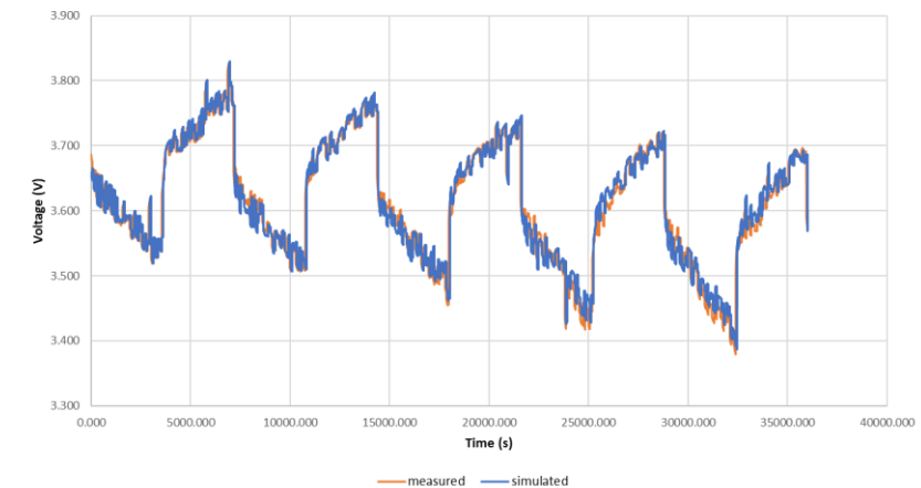
The comparison of the measured values of the test current profile with the model
