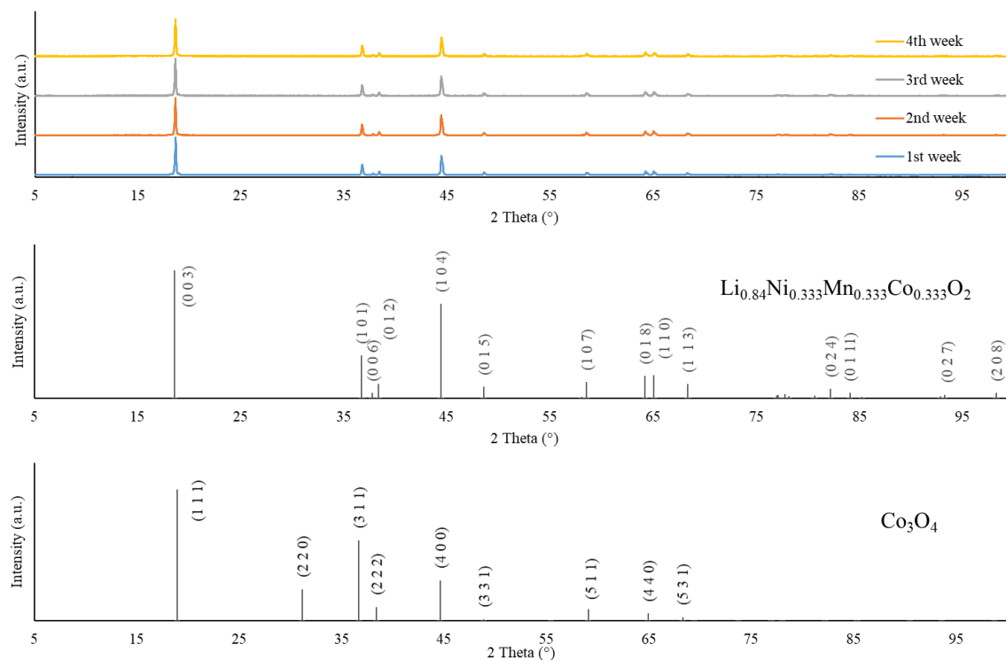
Figure 3: Diffractograms for NMC material
