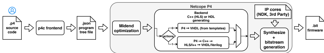
Figure 1: Compilation process
